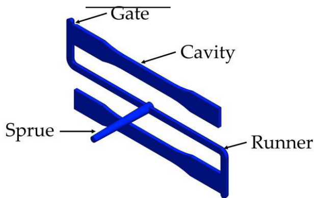
Figure 2. Fluid domain parts. Source: Project Author.
