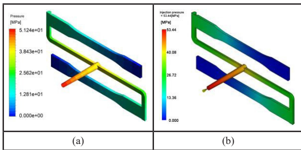
Figura 6. Result of the injection pressure required to fill the mold cavities: (a) Ansys® Workbench/Fluent module; (b) Moldflow® Adviser.
