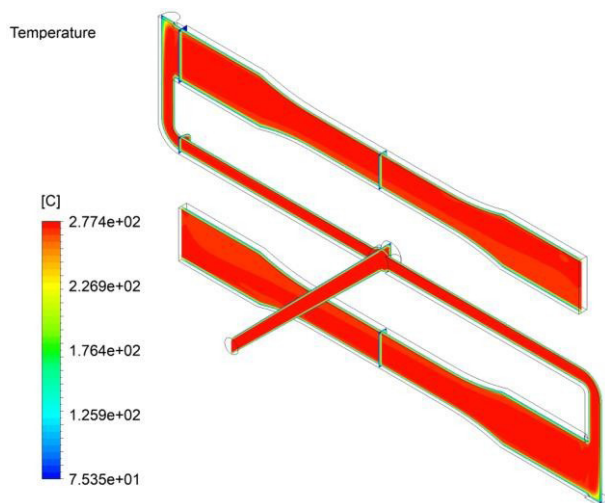
Figura 9. Flow front temperature results using Ansys® Workbench/Fluent module. Source: Project Author.
