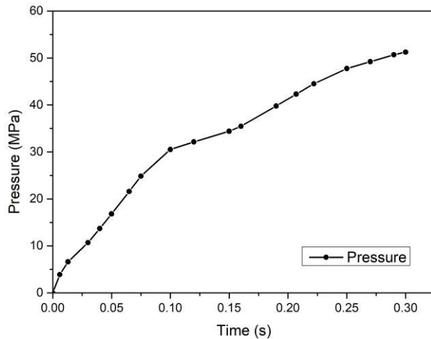
Figura 8. Inlet pressure profile over time. Source: Project Author.
