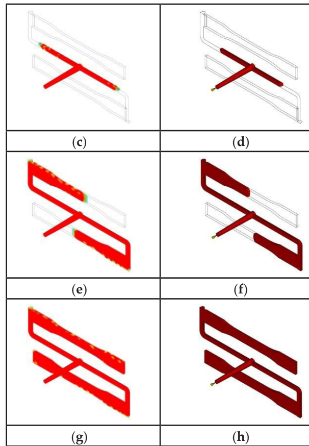
Figura 7. Polymer flow front visualization results over time: (a) Mold filling in time = 0.0130 s using Ansys® Workbench/Fluent module; (b) Mold filling in time = 0.0129 s using Moldflow® Adviser; (c) Mold filling in time = 0.0650 s using Ansys® Workbench/Fluent module; (d) Mold filling in time = 0.0645 s using Moldflow® Adviser; (e) Mold filling in time = 0.2070 s using Ansys® Workbench/Fluent module; (f) Mold filling in time = 0.2065 s using Moldflow® Adviser; (g) Mold filling in time = 0.3000 s using Ansys® Workbench/Fluent module; (h) Mold filling in time = 0.3097 s using Moldflow® Adviser.
