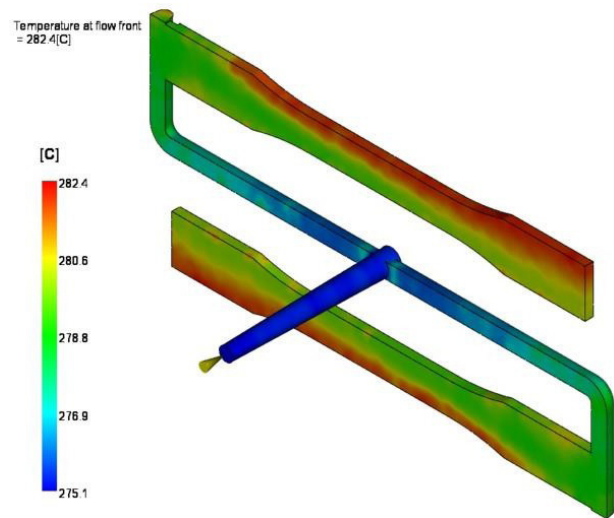
Figura 10. Flow front temperature results using Moldflow® Adviser. Source: Project Author.
