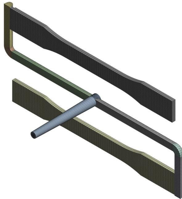
Figure 3. Fluid domain meshing. Source: Project Author. Source: Project Author.
