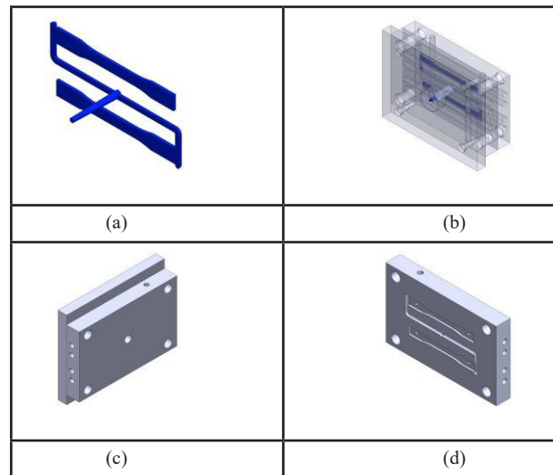
Figure 1. CAD models needed to simulate the injection molding process: (a) Fluid domain; (b) Assembled mold; (c) Fixed mold plate; (d) Mobile mold plate.
