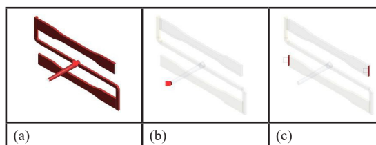
Figure 4. Boundary conditions for the injection phase: (a) Walls; (b) Inlet; (c) Outlets.
